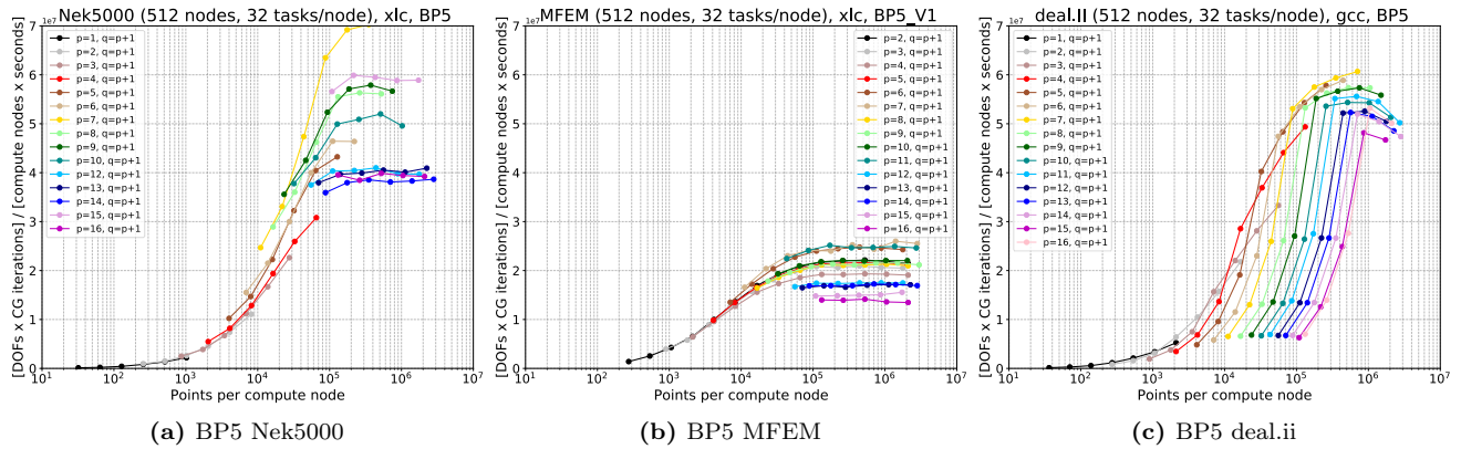
Figure 10: BP5 results of Nek5000 (left), MFEM (center), and deal.II (right) on BG/Q with varying polynomial order ( p = 1, \dots, 16 ) with the number of quadrature points ( q = p + 1 ). The number cpu cores P = 8,192 .
