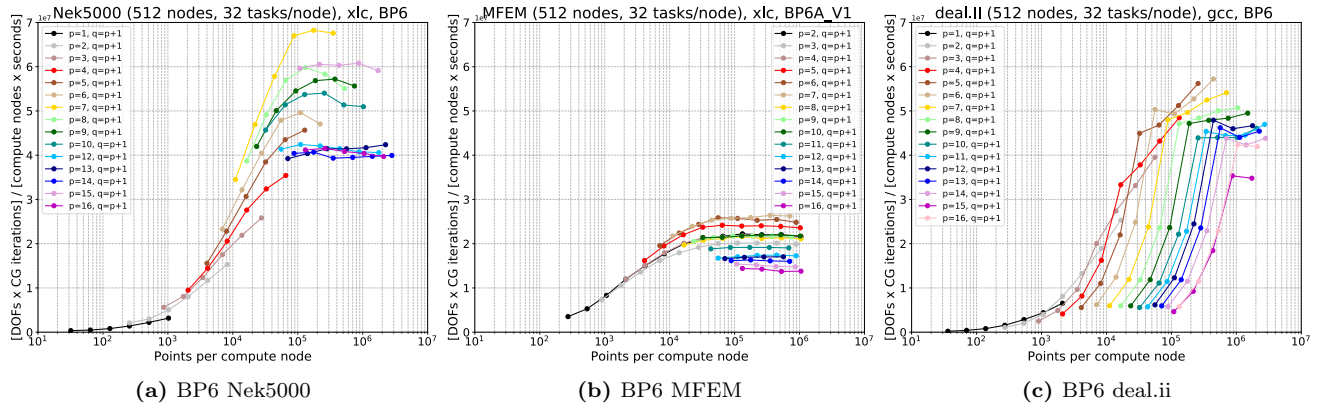
Figure 11: BP6 results of Nek5000 (left), MFEM (center), and deal.ii (right) on BG/Q with varying polynomial order ( p = 1, \dots, 16 ) with the number of quadrature points ( q = p + 1 ). The number CPU cores P = 8,192 .
