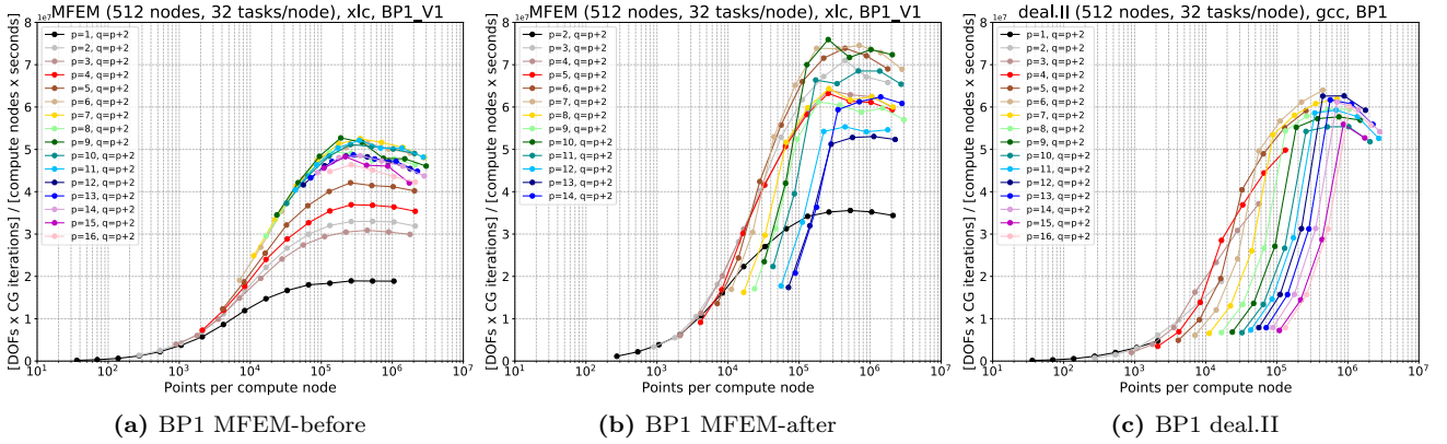
Figure 12: BP1 results of MFEM+xlc (left), MFEM+xlc+intrinsics (center), and deal.ii (right) on BG/Q with varying polynomial order ( p = 1, \dots, 16 ) with the number of quadrature points ( q = p + 2 ). The number cpu cores P = 8, 192 .
